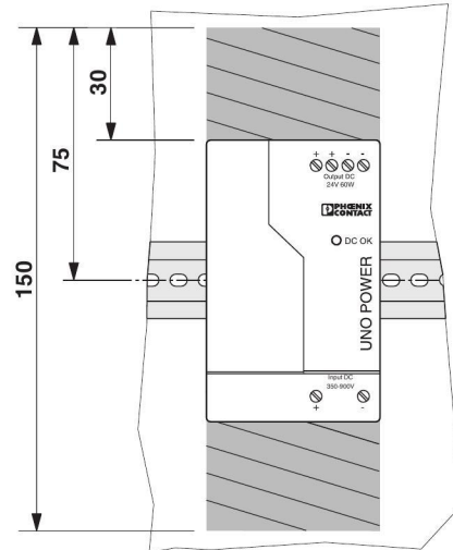
Figure 4 Locked areas
