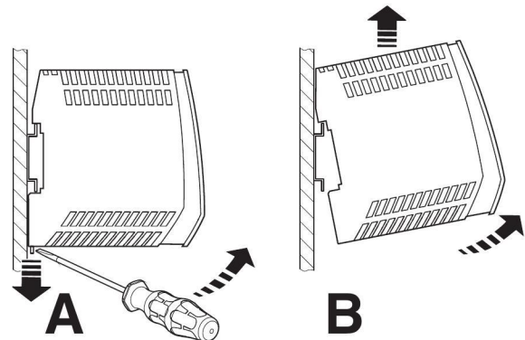
Figure 15 Removal
