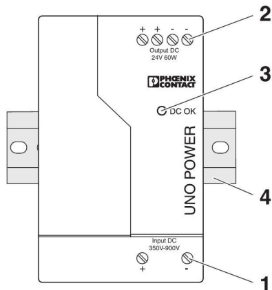
Figure 1 Device elements
